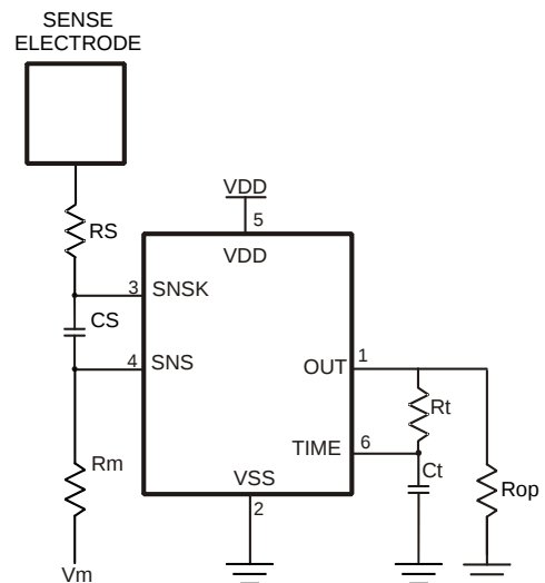
Figure 3.6 Programmable Delay
